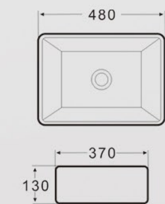
K58 Art Basin Size: 480x370x130mm Vareous China Above counter mountings
