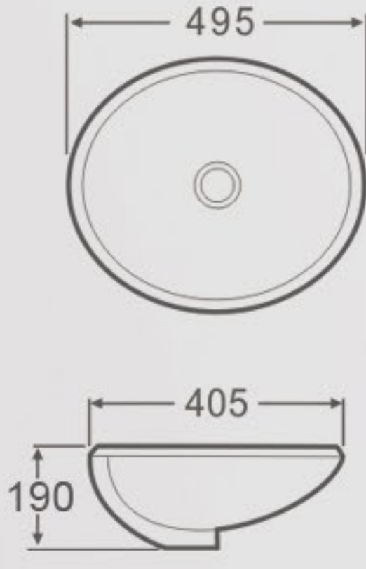
Y120 Under Counter Basin Size: 495x405x190mm Vareous China Under counter mountings
