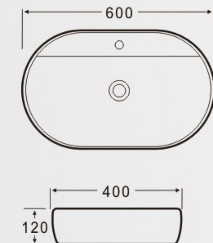
K431 Art Basin Size: 600x400x120mm Vareous China Above counter mountings
