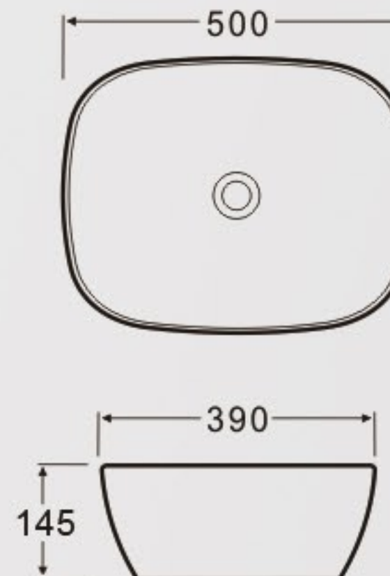
K435 Art Basin Size: 500x390x145mm Vareous China Above counter mountings
