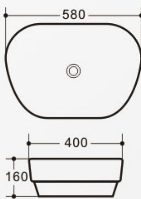
K489 Art Basin Size: 580x400x160mm Vareous China Above counter mountings
