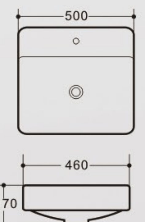
K493 Art Basin Size: 500x460x170mm Vareous China Semi-mounting
