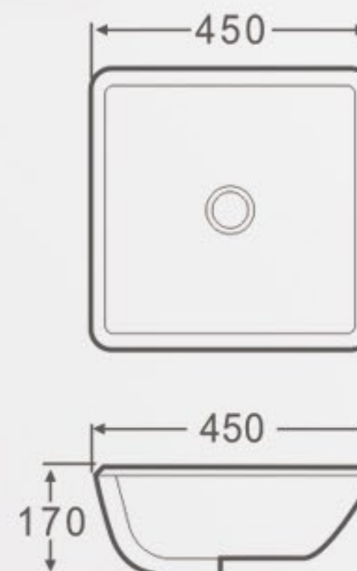
Y108 Under Counter Basin Size: 450x450x170mm Vareous China Under counter mountings
