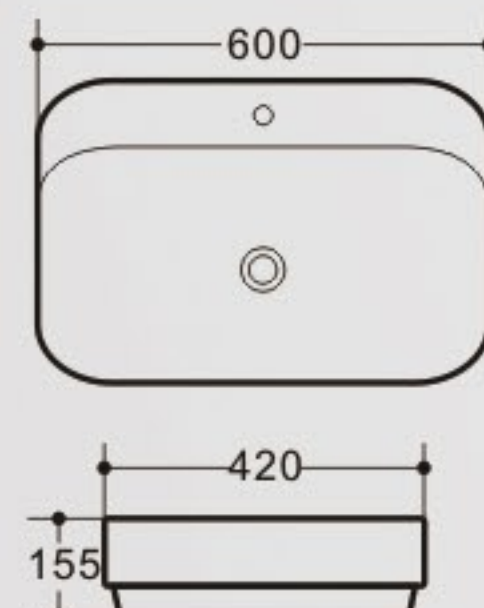
K487 Art Basin Size: 600x420x155mm Vareous China Above counter mountings
