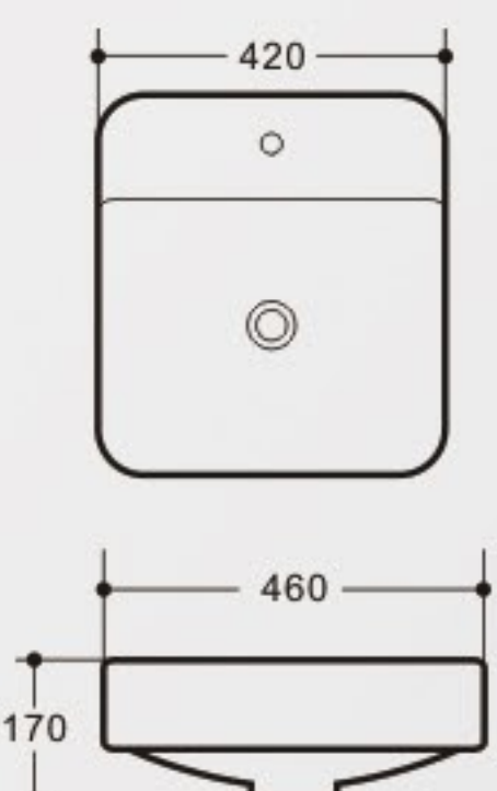
K492 Art Basin Size: 420x460x170mm Vareous China Semi-mounting
