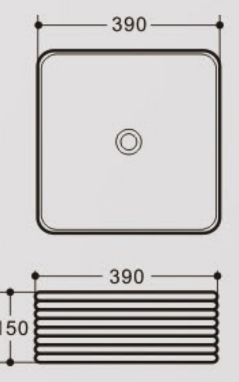
K451 Art Basin Size: 390x390x150mm Vareous China Above counter mountings
