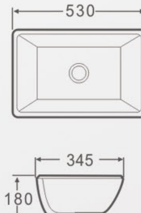
Y200A Under Counter Basin Size: 530x345x180mm Vareous China Under counter mountings
