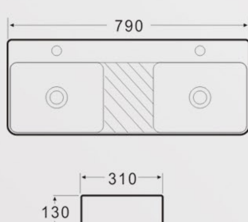
K537B Art Basin Size: 790x310x130mm Vareous China Above counter mountings
