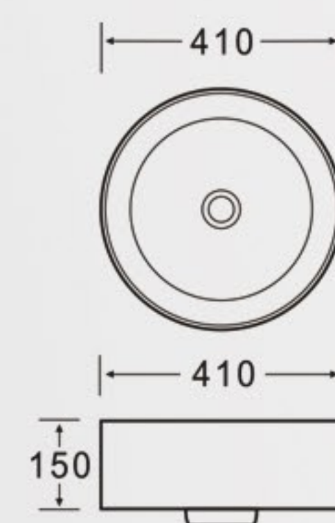
K539 Art Basin Size: 410x410x150mm Vareous China Above counter mountings
