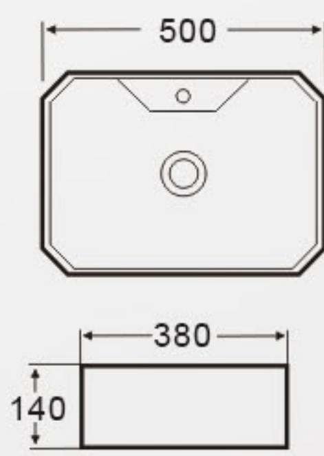
K445 Art Basin Size: 500x380x140mm Vareous China Above counter mountings
