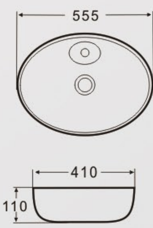
K448 Art Basin Size: 555x410x110mm Vareous China Above counter mountings
