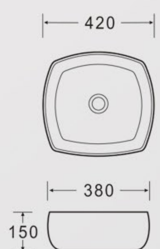
K542A Art Basin Size: 420x380x150mm Vareous China Above counter mountings
