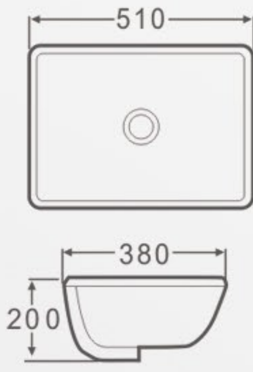
1633 Under Counter Basin Size: 510x380x200mm Vareous China Under counter mountings
