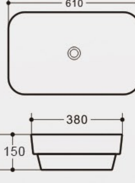
K491 Art Basin Size: 610x380x150mm Vareous China Above counter mountings
