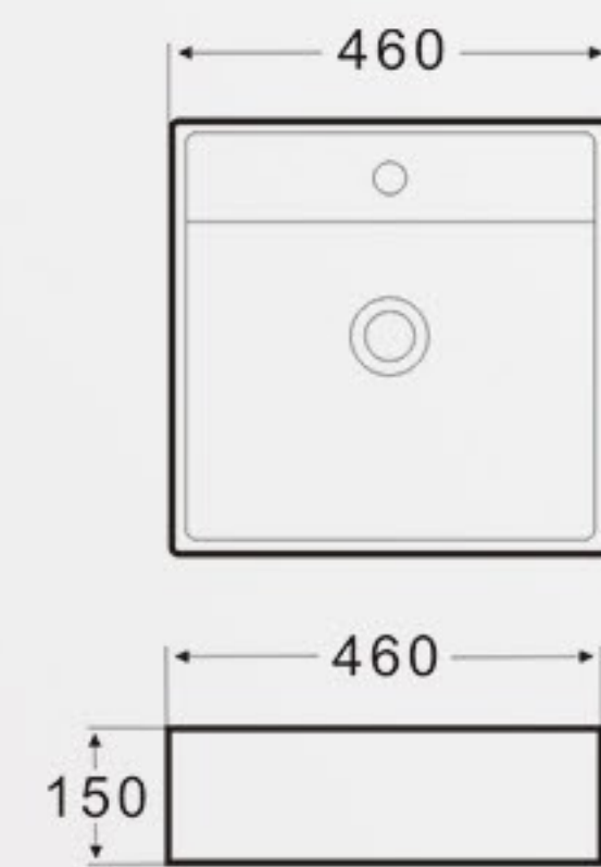
K49 Art Basin Size: 460x460x150mm Vareous China Above counter mountings / Wall-hung Installation
