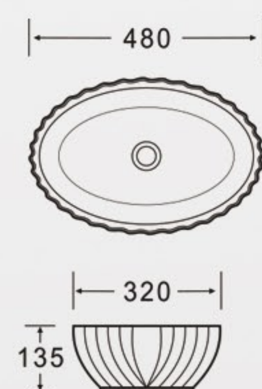
K541A Art Basin Size: 480x320x135mm Vareous China Above counter mountings
