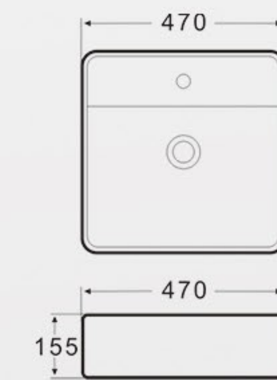
K55 Art Basin Size: 470x470x155mm Vareous China Above counter mountings
