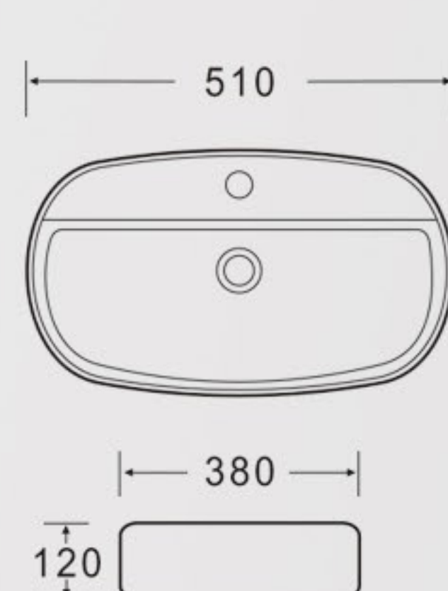
K543A Art Basin Size: 510x380x120mm Vareous China Above counter mountings
