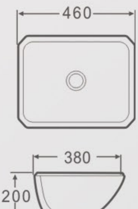
Y818 Under Counter Basin Size: 460x380x200mm Vareous China Under counter mountings
