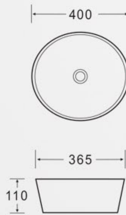
K538 Art Basin Size: 400x365x110mm Vareous China Above counter mountings
