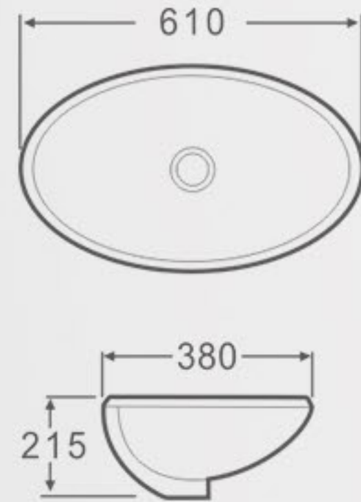
Y132 Under Counter Basin Size: 610x380x215mm Vareous China Under counter mountings
