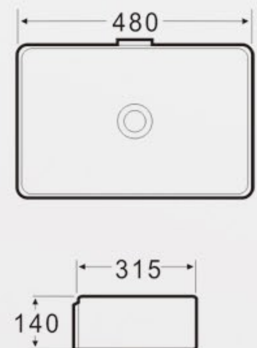
K536 Art Basin Size: 480x315x140mm Vareous China Above counter mountings
