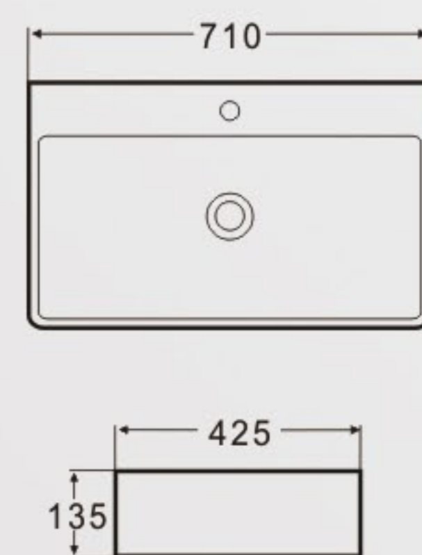
K427 Art Basin Size: 710x425x135mm Vareous China Above counter mountings / Wall-hung Installation
