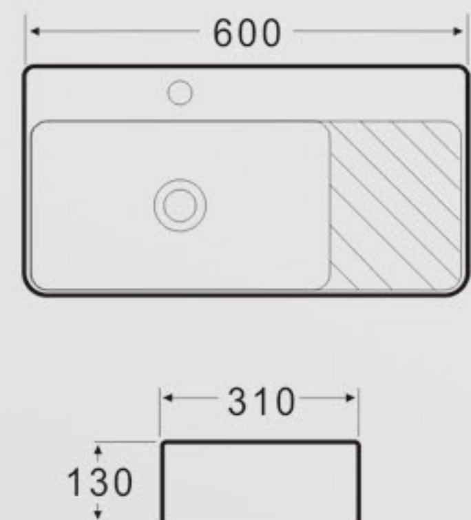
K537 Art Basin Size: 600x310x130mm Vareous China Above counter mountings
