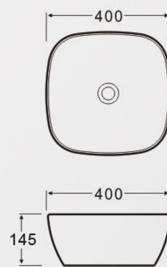
K434 Art Basin Size: 400x400x145mm Vareous China Above counter mountings
