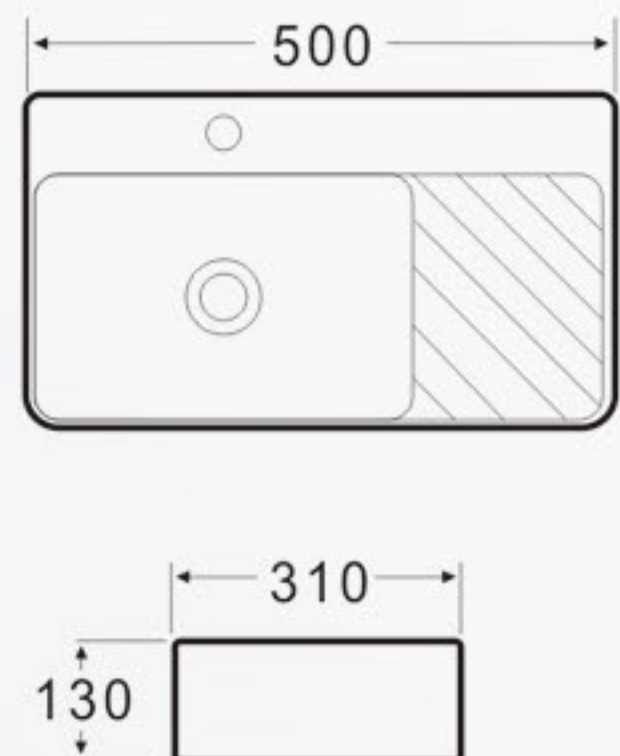
K537A Art Basin Size: 500x310x130mm Vareous China Above counter mountings
