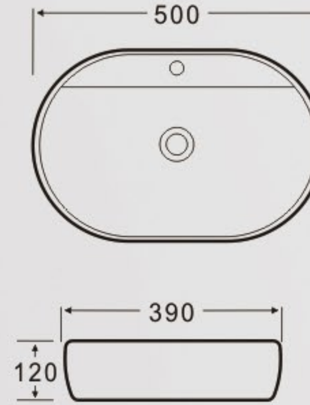
K430 Art Basin Size: 500x390x120mm Vareous China Above counter mountings
