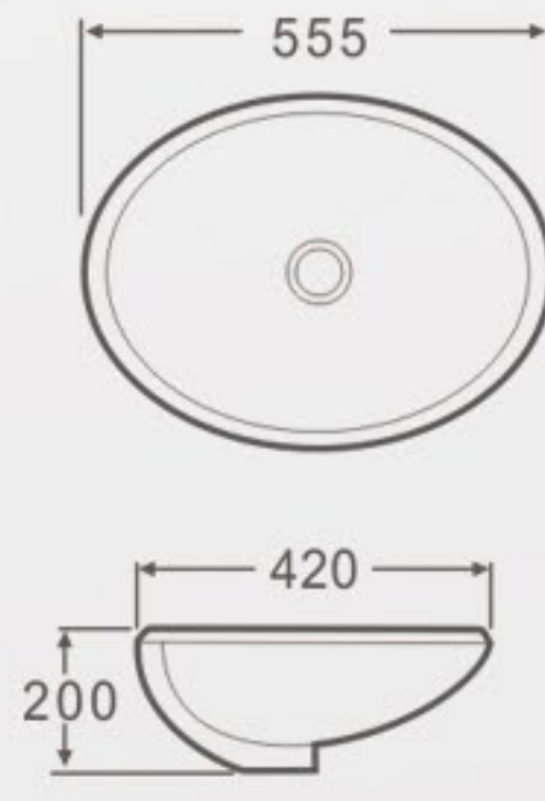
Y222 Under Counter Basin Size: 555x420x200mm Vareous China Under counter mountings
