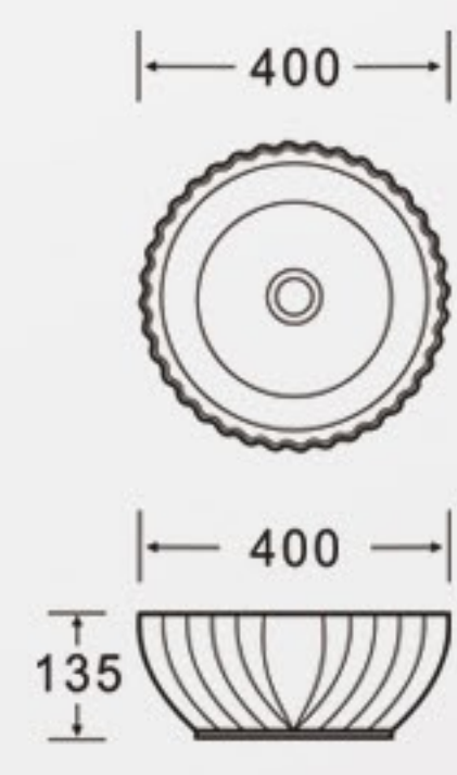
K541 Art Basin Size: 400x400x135mm Vareous China Above counter mountings
