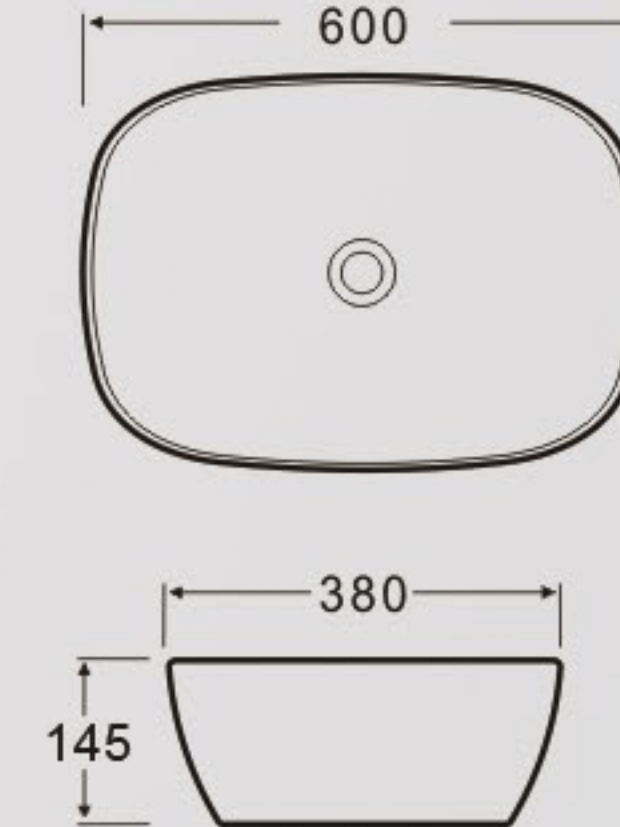
K436 Art Basin Size: 600x380x145mm Vareous China Above counter mountings
