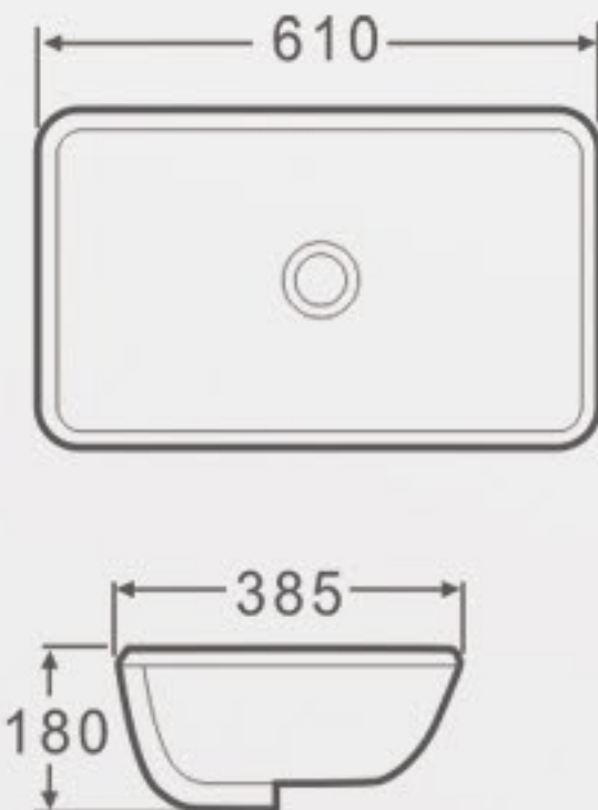
1610 Under Counter Basin Size: 610x385x180mm Vareous China Under counter mountings
