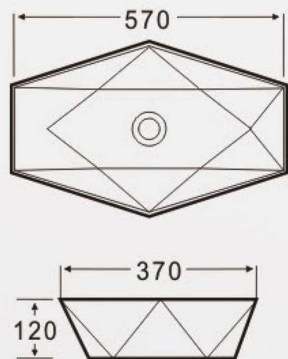
K423 Art Basin Size: 570x370x120mm Vareous China Above counter mountings
