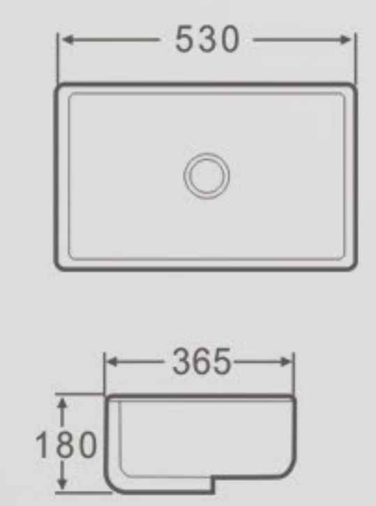
Y109 Under Counter Basin Size: 530x365x180mm Vareous China Under counter mountings
