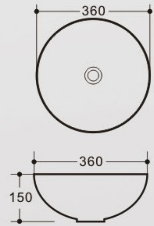
K449 Art Basin Size: 360x360x150mm Vareous China Above counter mountings
