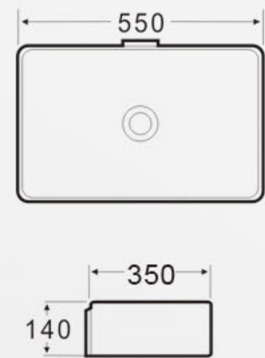
K536B Art Basin Size: 550x350x140mm Vareous China Above counter mountings
