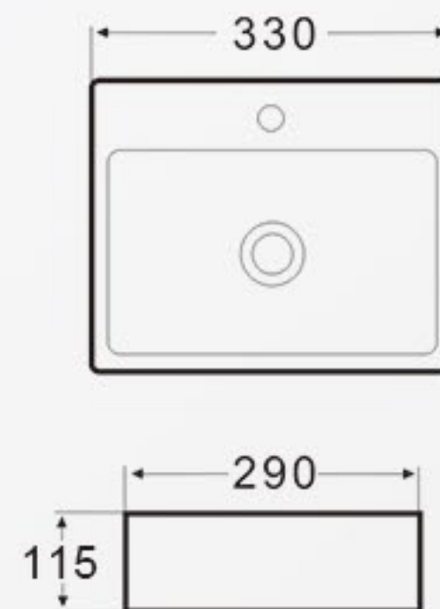
K51 Art Basin Size: 330x290x115mm Vareous China Above counter mountings / Wall-hung Installation
