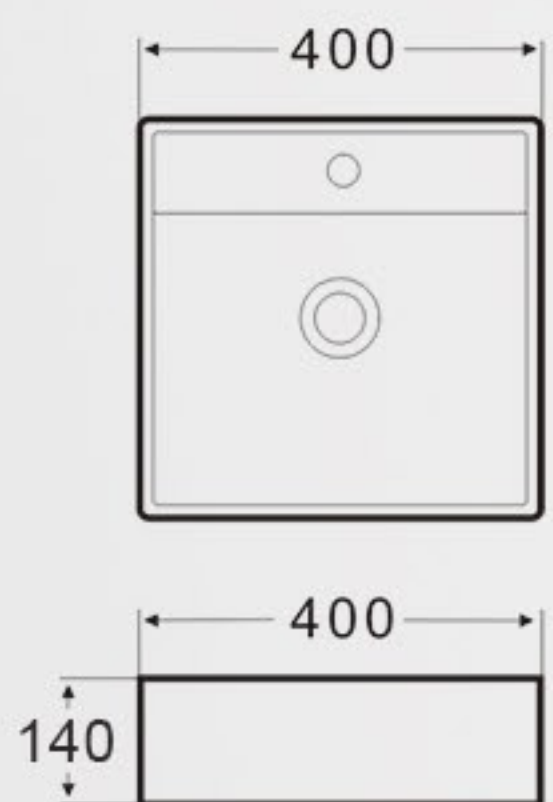
K49A Art Basin Size: 400x400x140mm Vareous China Above counter mountings / Wall-hung Installation
