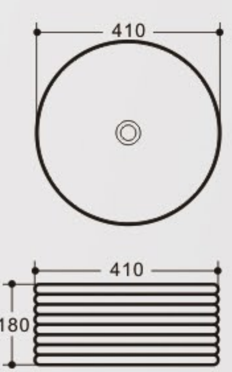
K450 Art Basin Size: 410x410x180mm Vareous China Above counter mountings
