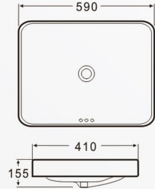
K425 Art Basin Size: 590x410x155mm Vareous China Semi-mounting
