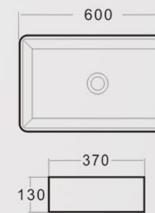
K58A Art Basin Size: 600x370x130mm Vareous China Above counter mountings
