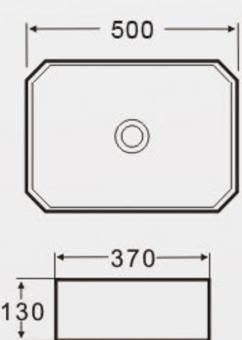
K446 Art Basin Size: 500x370x130mm Vareous China Above counter mountings
