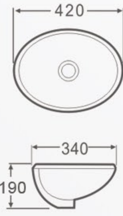
Y016 Under Counter Basin Size: 420x340x190mm Vareous China Under counter mountings
