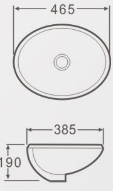
Y518 Under Counter Basin Size: 465x385x190mm Vareous China Under counter mountings
