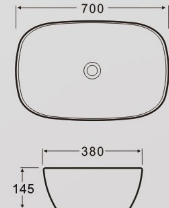
K437 Art Basin Size: 700x380x145mm Vareous China Above counter mountings
