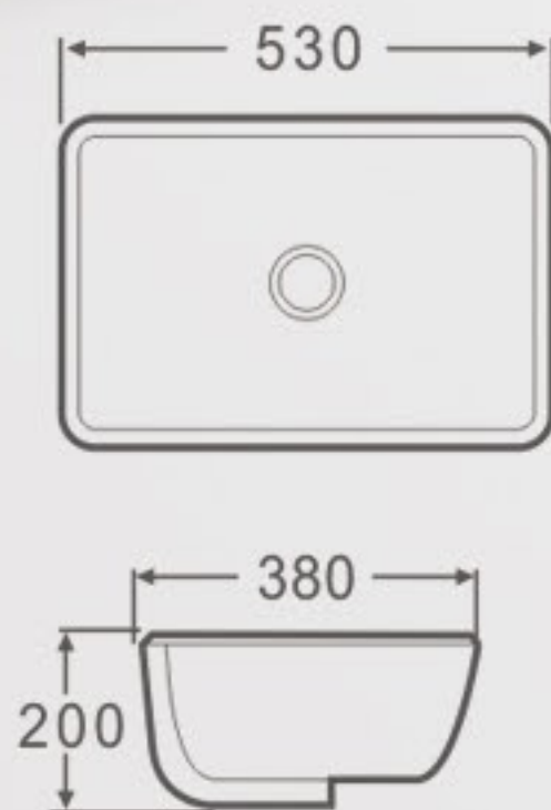
Y107 Under Counter Basin Size: 530x380x200mm Vareous China Under counter mountings
