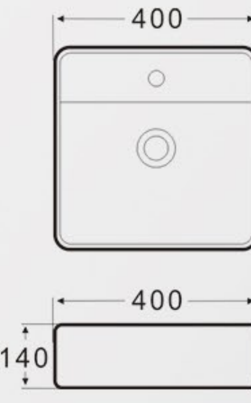
K55A Art Basin Size: 400x400x140mm Vareous China Above counter mountings / Wall-hung Installation
