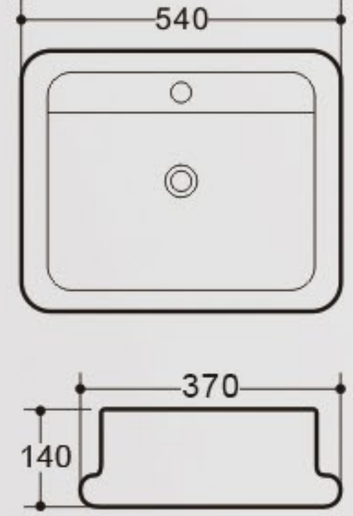
K440 Art Basin Size: 540x370x140mm Vareous China Above counter mountings
