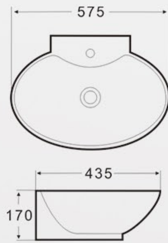
K42 Art Basin Size: 575x435x170mm Vareous China Above counter mountings / Wall-hung Installation
