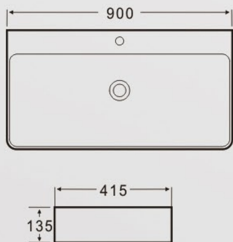
K426 Art Basin Size: 900x415x135mm Vareous China Above counter mountings / Wall-hung Installation
