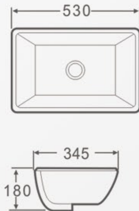
Y200 Under Counter Basin Size: 530x345x180mm Vareous China Under counter mountings
