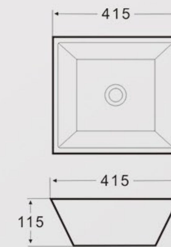
K57 Art Basin Size: 415x415x115mm Vareous China Above counter mountings
