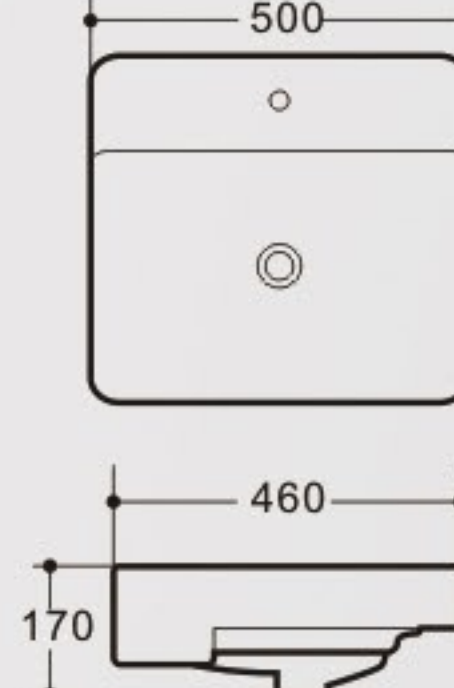
K493B Art Basin Size: 500x460x170mm Vareous China Semi-mounting
