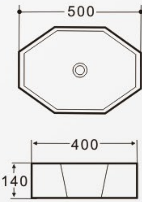
K442 Art Basin Size: 500x400x140mm Vareous China Above counter mountings
