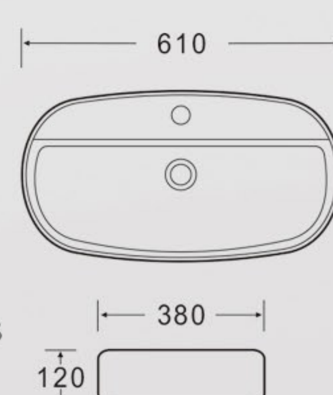
K543 Art Basin Size: 610x380x120mm Vareous China Above counter mountings
