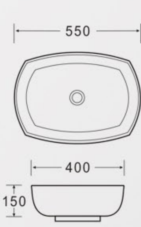
K542 Art Basin Size: 550x400x150mm Vareous China Above counter mountings
