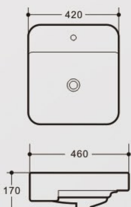
K492B Art Basin Size: 420x460x170mm Vareous China Semi-mounting
