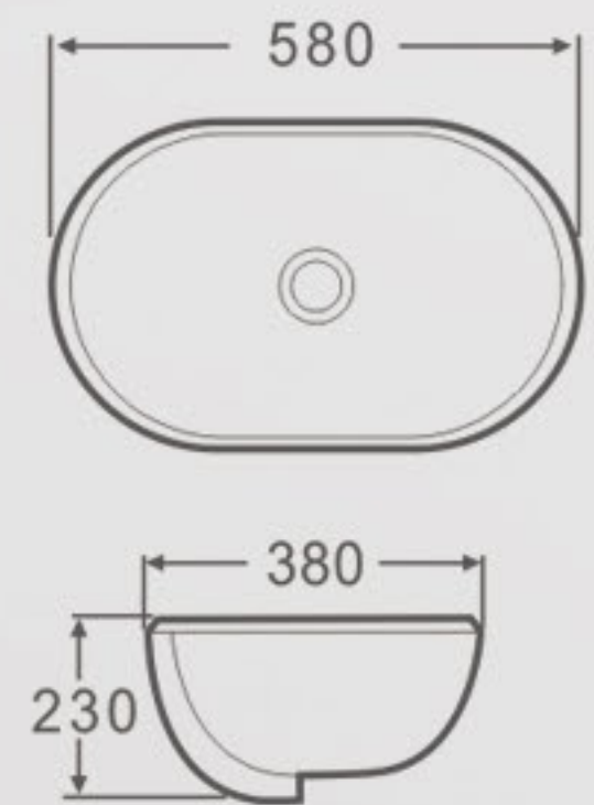
Y028 Under Counter Basin Size: 580x380x230mm Vareous China Under counter mountings
