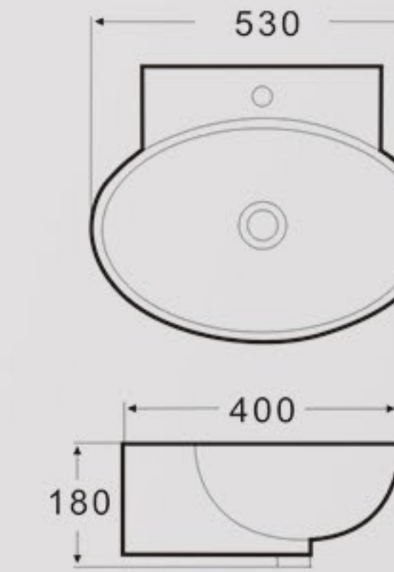
K59 Art Basin Size: 530x400x180mm Vareous China Wall-hung Installation
