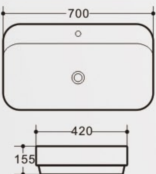
K488 Art Basin Size: 700x420x155mm Vareous China Above counter mountings
