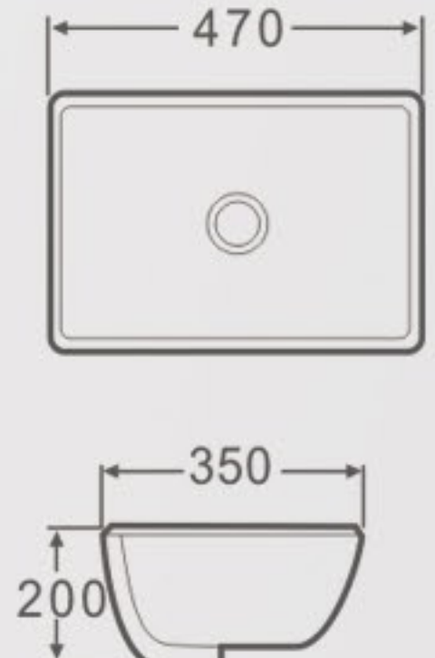
Y918 Under Counter Basin Size: 470x350x200mm Vareous China Under counter mountings
