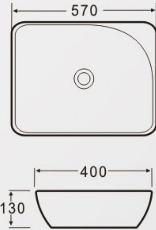
K447 Art Basin Size: 570x400x130mm Vareous China Above counter mountings
