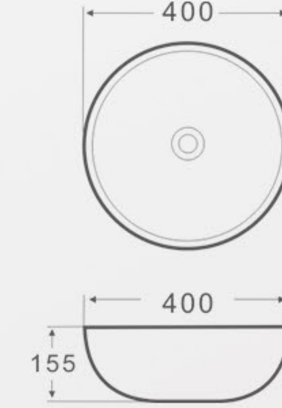
K53 Art Basin Size: 400x400x155mm Vareous China Above counter mountings
