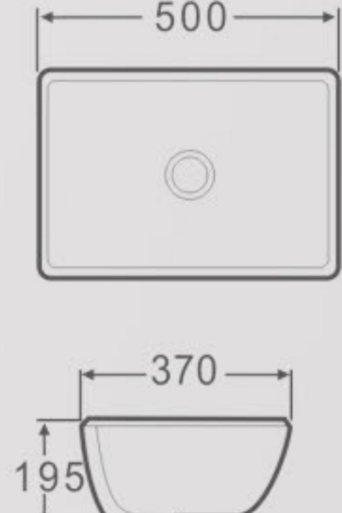
Y919 Under Counter Basin Size: 500x370x195mm Vareous China Under counter mountings
