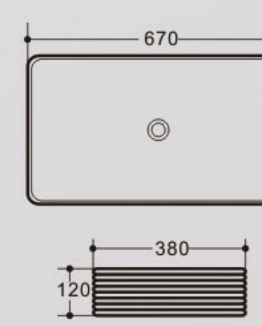
K452 Art Basin Size: 670x380x120mm Vareous China Above counter mountings
