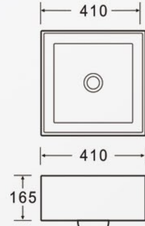
K540 Art Basin Size: 410x410x165mm Vareous China Above counter mountings
