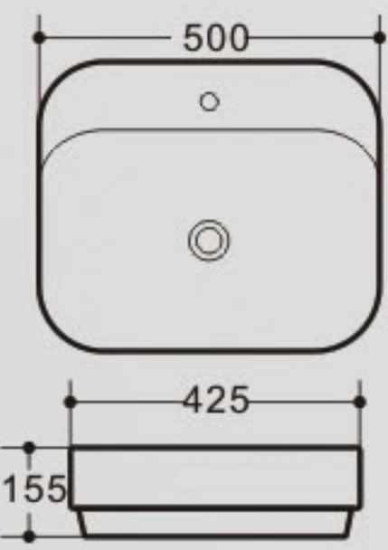
K486 Art Basin Size: 500x425x155mm Vareous China Above counter mountings
