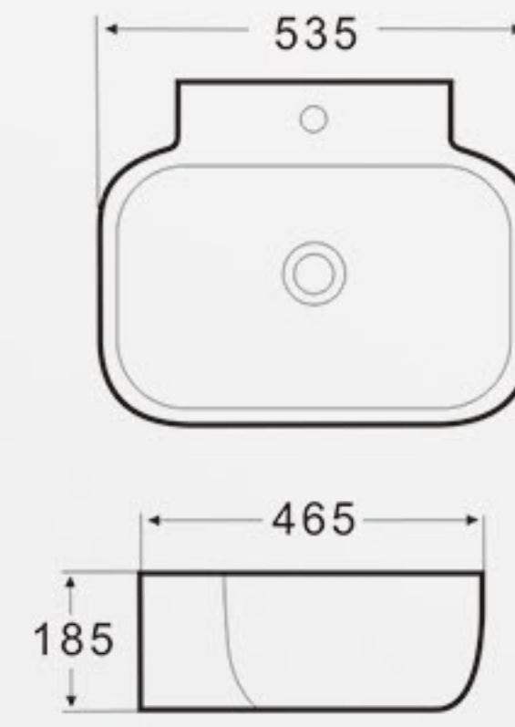
K44 Art Basin Size: 535x465x185mm Vareous China Wall-hung Installation
