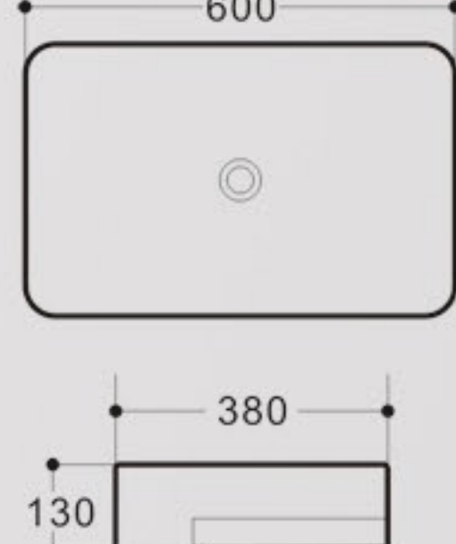
K494 Art Basin Size: 600x380x130mm Vareous China Semi-mounting
