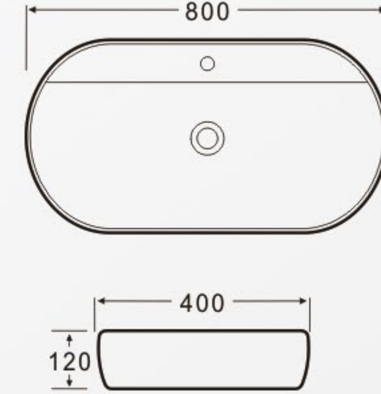
K432 Art Basin Size: 800x400x120mm Vareous China Above counter mountings
