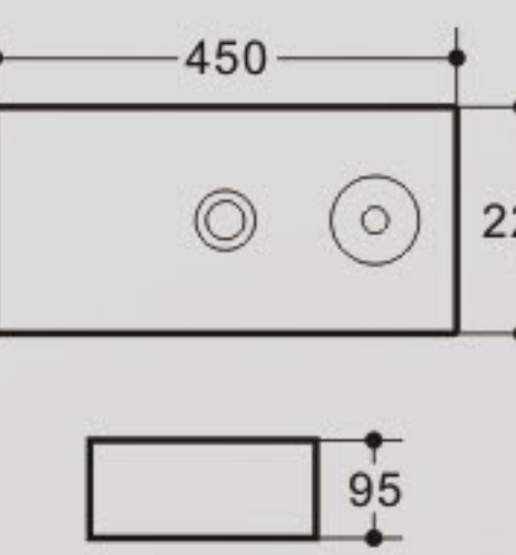
K495 Art Basin Size: 450x220x95mm Vareous China Above counter mountings
